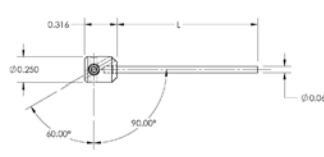
H - 60/90 (TUNGSTEN HOLDER ASSEMBLY 60 & 90 DEG. P/N 002-0771)
