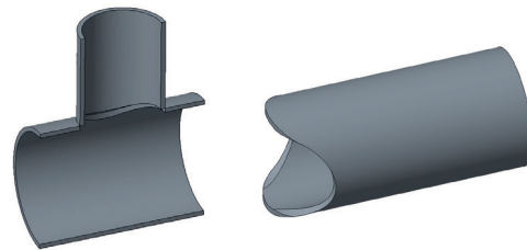
BRANCH SITTING ON MAIN PIPE
